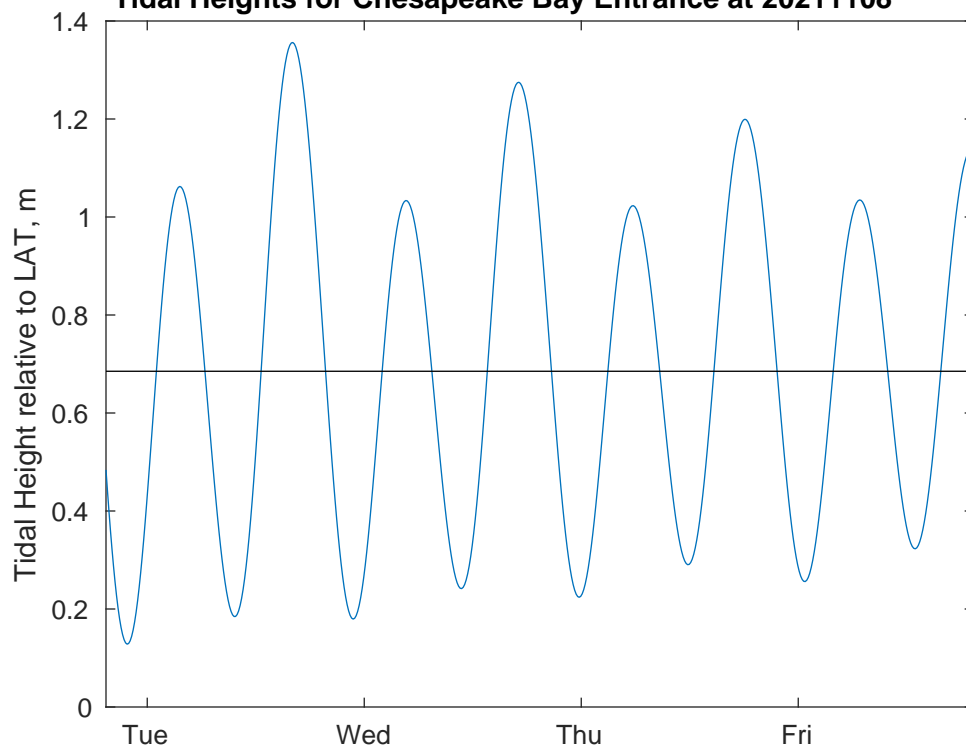
Tidal Heights for Chesapeake Bay Entrance at 20211108
